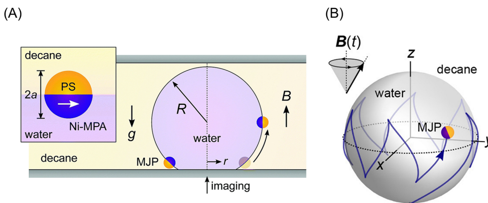
Fig. 8 (A) Schematic illustration of a magnetic Janus particle (MJP) moving on the curved interface of a water droplet in decane due to a homogeneous magnetic field B . The inset shows the preferred orientation of the MJP at the interface and its magnetic moment (white arrow). Reproduced from ref. 108 with permission from The Royal Society of Chemistry. (B) Simulation of zig-zag motion of MJP in the interface due to a precessing magnetic field. Reprinted with permission from ref. 110. Copyright © 2020, the American Chemical Society.
