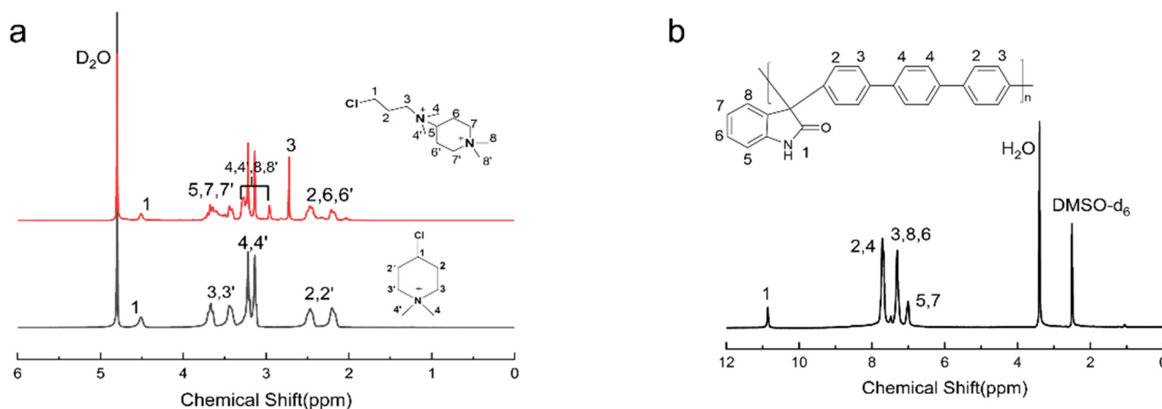
Fig. 1 ^1\text{H} NMR spectra of (a) 4-ClPq and 3-N-4-CIPq; (b) poly( p -terphenyl isatin).
