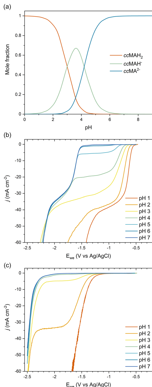
Fig. 2 (a) Speciation diagram for ccMA calculated for pK_{a1} = 3.0 and pK_{a2} = 4.2 ; ccMAH 2 , ccMAH - , and ccMA 2- correspond to diprotic, monoprotic, and fully deprotonated species. (b and c) pH-Dependent current–potential polarization curves on Pb RDE for 0.1 M K 2 SO 4 /H 2 SO 4 (b) with 0.5 g L -1 ccMA and (c) without ccMA.
