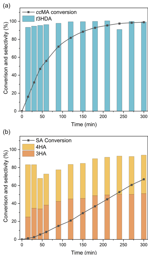
Fig. 6 Conversion and selectivity achieved for the bulk electrolysis of (a) cis,cis -muconic acid ( ccMA ), and (b) sorbic acid ( SA ) in a divided flow reactor operated at a constant current of 100 mA cm -2 . ccMA only produced trans -3-hexenedioic acid ( t 3HDA) while SA produced 3-hexenoic acid (3HA) and 4-hexenoic acid (4HA).
