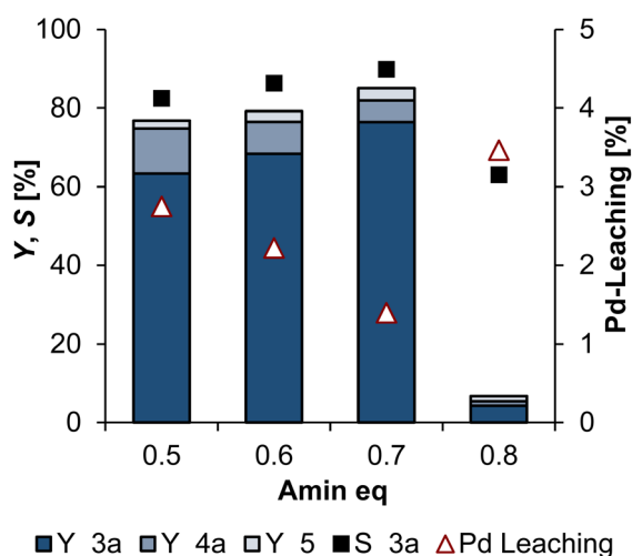
Fig. 7 Results for different diethylamine equivalents in the telomerisation of \beta -myrcene ( 1 ) with diethylamine ( 2a ). Conditions: 20 mmol \beta -myrcene ( 1 ), HNEt 2 ( 2a ), 0.035 mol% Pd(acac) 2 , 0.14 mol% TPPTS, P: Pd: 4:1, EtOH: H 2 O (w/w) 70:30, 1: solvent (w/w) 1:1, 1 bar Ar, 100 °C, 4 h, 500 rpm. Yield (Y), and selectivity (S) determined by GC-FID with n -dodecane as internal standard; leaching determined by ICP-OES and calculated as the amount lost with respect to the initial amount of palladium.
