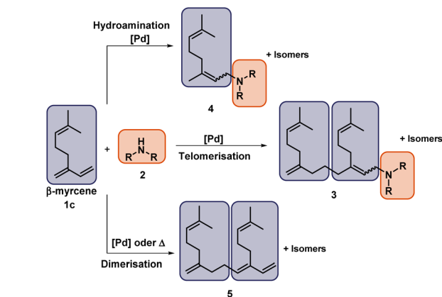
Fig. 2 Reaction network of the telomerisation of \beta -myrcene ( 1 ) with an amine ( 2 ). R = H, alkyl, aryl.
