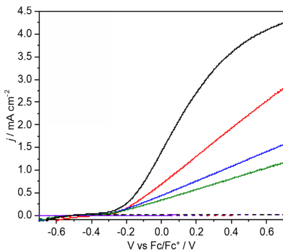
Fig. 2 Linear sweep voltammograms of BiVO 4 photoelectrodes in electrolytes containing 2 M (black line), 1 M (red), 0.5 M (blue), 0.25 M (green), and 0.01 M (purple) PAA with 0.05 equiv. NEt 3 . Voltammograms were recorded in the dark (dashed) and under 450 nm LED illumination (solid). Scan rate 10 mV s -1 .
