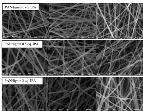
Fig. 9 SEM images of electrospun fibers (left), after thermostabilization (middle; T = 250\text{ }^\circ\text{C} for t = 1\text{ h} at 0.5\text{ }^\circ\text{C min}^{-1} ), and carbonization (right; T = 1000\text{ }^\circ\text{C} at 5\text{ }^\circ\text{C min}^{-1} ) steps using acetylated lignin with different amounts of iPac and s-OH. Adapted with permission from ref. 178. Copyright 2021 Elsevier Ltd.
