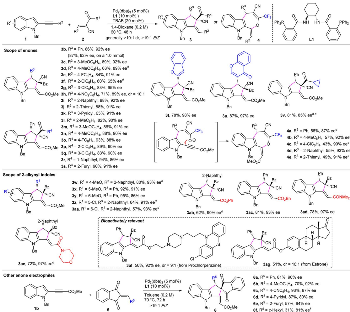
Scheme 2 Substrate scope of the asymmetric [3+2] or [3+4] annulation reaction of 2-alkynyl indoles and enones. a,b,c Unless noted otherwise, reactions were carried out with indole 1 (0.10 mmol), enone 2 (0.13 mmol) or 5 (0.12 mmol), \text{Pd}_2(\text{dba})_3 (5 mol%), L1 (10 mol %), and TBAB (20 mol%) in solvent (0.5 mL) under Ar for 48 h. b Yield of the isolated product. c Determined by HPLC analysis on a chiral stationary phase. d With 2 (1.5 equiv) at 80 °C. e Without TBAB. f At 90 °C for 5d . The absolute configuration of enantiopure 3i , 6c and the structure of rac - 4d was determined by X-ray analysis. The other products were assigned by analogy.
