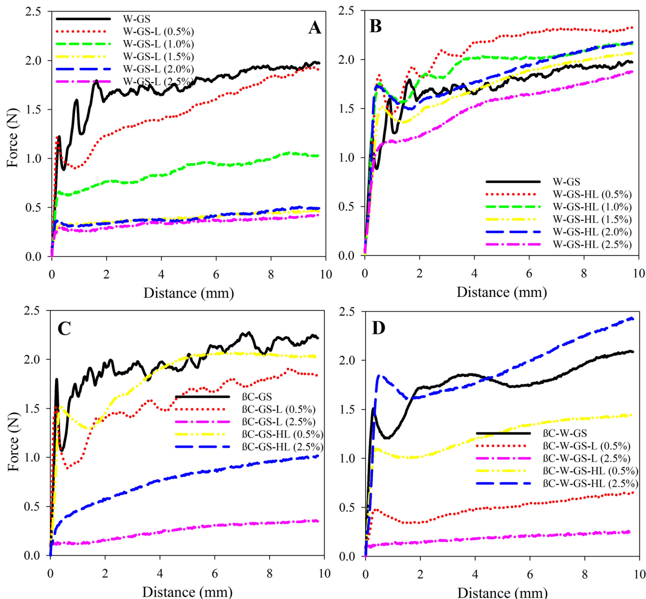
Fig. 5 Penetration force (N) of water (W)-filled (1% w/w) and \beta -carotene ( \beta C) (0.1% w/w)-enriched corn oil oleogels over 10 mm of distance and at 25.0 \pm 0.1 °C for mixed systems with glyceryl stearate (GS) 20% (w/w) and varying concentrations of lecithin (L) or hydrogenated lecithin (HL) (0 to 2.5% w/w): water-filled lecithin-containing oleogels (A), water-filled hydrogenated lecithin-containing oleogels (B), enriched oleogels with \beta C (C), and water-filled oleogels enriched with \beta C (D).
