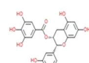
Epigallocatechin 3-O-gallate [3]
