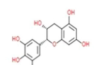
Epigallocatechin [1]
