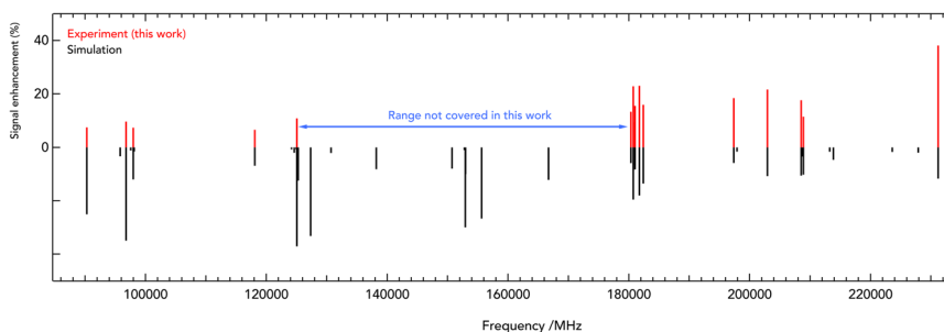
Fig. 3 Stick spectra of the pure rotational transitions of \text{c-C}_3\text{H}_2\text{D}^+ measured between 90 and 230 GHz. The experimental frequencies (in red, top) are compared to a PGOPHER simulation at 10 K (black, bottom). The experimental intensities are given as signal enhancement of the normalized ion counts (as in Fig. 2). The regions 90–125 GHz and 175–230 GHz were collected using two different multiplier chain settings and no experimental measurement was done for 125–170 GHz.
