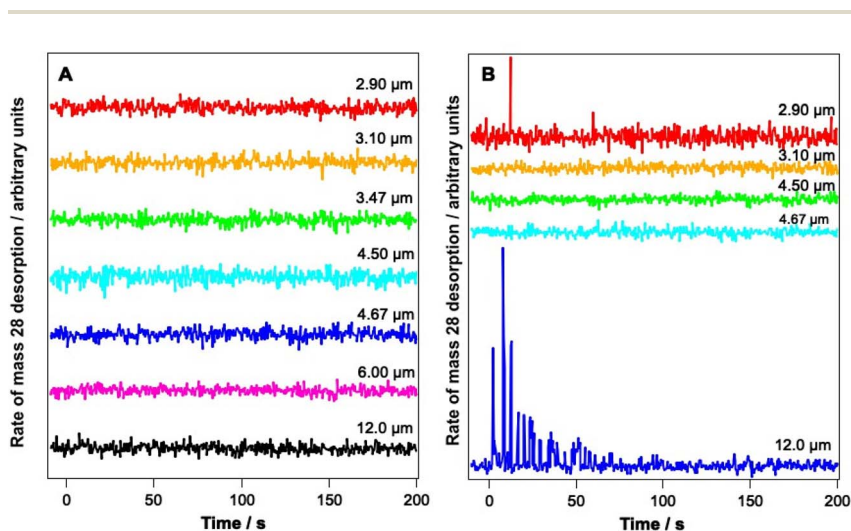
Fig. 4 PID traces recorded during irradiation of (A) a 6.25% CO–water mixed ice and (B) a 41.7% CO–water mixed ice with light of various wavelengths for a total of 5 minutes. Ices were dosed onto Au-coated Cu at 18 K. Time 0 s represents the time at which the irradiation began.
