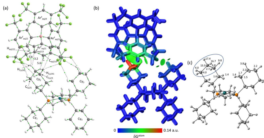
Fig. 8 (a) QTAIM molecular graph with Eq-2 in [1-propane][BAR F 4 ] with BCPs in green and showing selected atoms and BCP electron densities (a.u. × 10 −3 ). Bond paths with \rho(r) < 0.001 a.u., intramolecular bond paths and ring critical points (RCP) are omitted for clarity. (b) IGMH plot where the cation and anion are defined as separate fragments. Sign( \lambda_2 ) \rho -coloured isosurfaces are plotted with \delta G^{\text{inter}} = 0.003 a.u. and atoms are coloured by \delta G^{\text{atom}} . (c) \% \delta G^{\text{atom}} contributions on the cation that are above 1%, with the propylene motif highlighted (see text for details).
