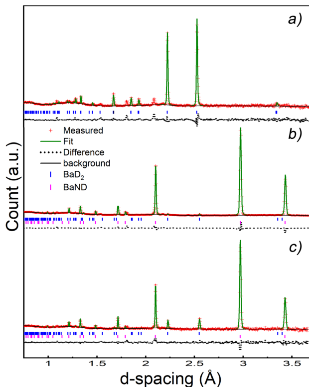
Fig. 9 NPD patterns: (a) starting pattern refined with the HT BaD 2 phase. (b) Pattern 120 ( i.e. the middle of the experiment) refined with a HT BaD 2 phase and a BaND phase. The refinement gave an 80% concentration of BaND by weight. (c) Last 73 patterns summed and refined with a BaD 2 and BaND phase. The refinement gave a 96% concentration of BaND by weight.
