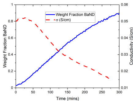
Fig. 10 Trend in calculated conductivity and phase fraction of BaND for doping of \text{BaD}_2 with \text{N}_2 experimentally. The emergence of BaND is associated with a decrease in conductivity. Beyond 280 min, the resistance associated with the high frequency response increases dramatically making the accurate modelling of the R_s difficult.
