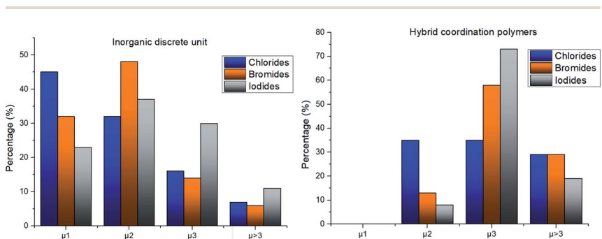
Fig. 2 Percentage of the coordination number of the different halides in the structures that have inorganic discrete units and percentage of the coordination number of the different halides in the hybrid coordination polymers.
