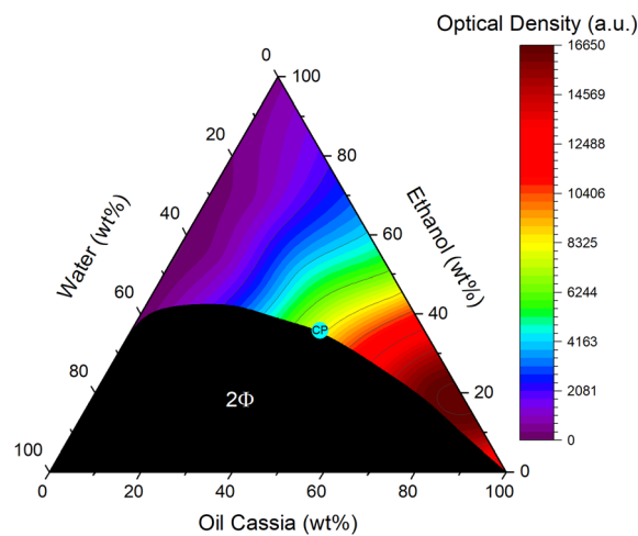
Fig. 4 Ternary phase diagram of water, ethanol, and Cinnamomum cassia oil (PCW). The black region labelled 2\Phi marks the two-phasic region. The heat map of the monophasic domain shows the solubility of curcumin with red indicating a high solubility while purple shows a low one. The critical point of the mixture is signified by the turquoise circle labelled CP.
