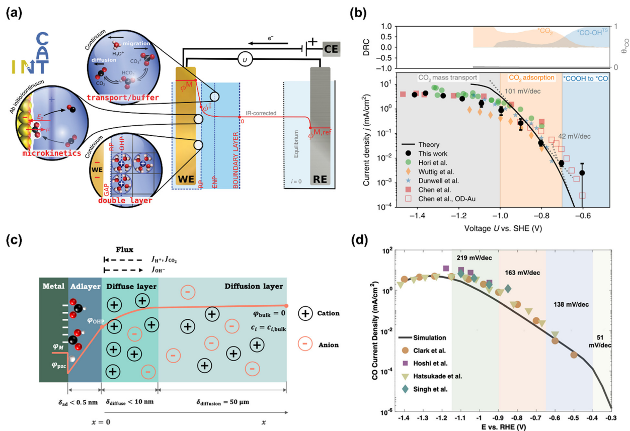
Fig. 5 (a) Schematic illustration of the multi-scale system. (b) Multi-scale \text{CO}_2 electroreduction simulation results over Au compared with experiments. Reproduced with permission. 32 Copyright 2020, Nature publishing group. (c) Schematic illustration of the model system. (d) Multi-scale \text{CO}_2 electroreduction simulation results over Ag compared with experiments. Reproduced with permission. 97 Copyright 2021, American Chemical Society.
