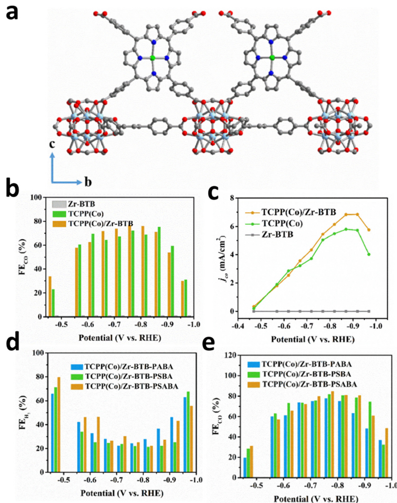
Fig. 18 (a) Schematic diagram of TCPP(Co)/Zr-BTB. (b) FE_{CO} and (c) CO j_p for all catalysts at different applied voltages. (d) FE_{H_2} and (e) FE_{CO} for PABA-, PSBA-, and PSBA-modified TCPP(Co)/Zr-BTB at different potentials. Reproduced with permission. 18 Copyright (2019) Wiley-VCH.
