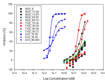
Fig. 2 Dose–response curves (DRCs) for A. fischeri growth inhibition of single metal oxide nanoparticles (MONPs). ZnO (blue lines), TiO 2 anatase (red lines), TiO 2 rutile (green lines), and SiO 2 (black lines).
