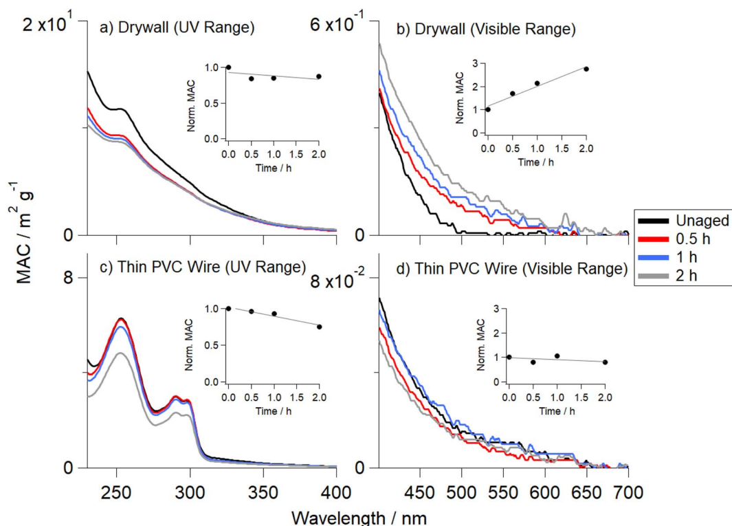
Fig. 2 Wavelength-dependent MAC values recorded after photolysis on Teflon filters and the subsequent extractions of drywall OA (a) and thin PVC wire OA (c) and (d). Each quarter of the filter was aged separately for 0.5 h (red), 1 h (blue), or 2 h (gray) and is compared with the unaged (0 h) fraction (black). The integrated MAC values (normalized to the unaged value) are shown as a subplot in each panel, with the UV integrated over 280–400 nm and the visible integrated over 400–700 nm. Boxcar averaging of the MAC data (over a 5 nm range) was utilized to improve signal-to-noise ratio.
