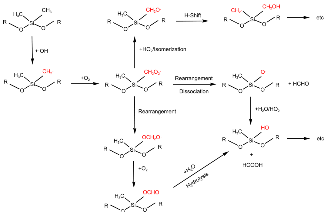
Fig. 3 Example reaction pathways of the OH-initiated oxidation of D_5 -siloxane (R represents the either side of the central silicon atom).
