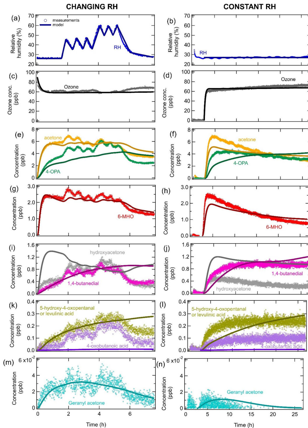
Fig. 5 Measurements (markers) and model outputs (lines) of the temporal evolution of (a and b) RH, (c and d) ozone, and (e–n) gas-phase ozonolysis products after four soiled T-shirts are exposed to ozone under (left hand side panels) changing RH conditions and (right hand side panels) constant RH as part of the ICHEAR experiments. All measurements have had the background concentrations subtracted for simplicity when modeling. Measurements for the changing RH conditions are from Arata et al. 24 and were performed at a temperature of 27.4–28.3 °C. The data at a constant RH is from ICHEAR experiments performed on the 19–20 May 2019.
