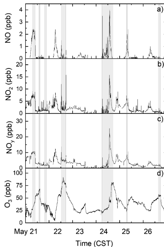
Fig. 3 Air quality ground station observations of (a) \text{NO} (ppb), (b) \text{NO}_2 (ppb), (c) \text{NO}_y (ppb) and (d) \text{O}_3 (ppb) at Chiwaukie Prairie from May 21–26, 2021. Lake breeze or onshore flow from SSE is highlighted as grey bars.
