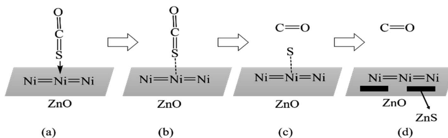
Fig. 13 Desulfurization mechanism of reduced Ni and COS reactions (this figure has been adapted/reproduced from ref. 108 with permission from Elsevier, copyright 2015).
