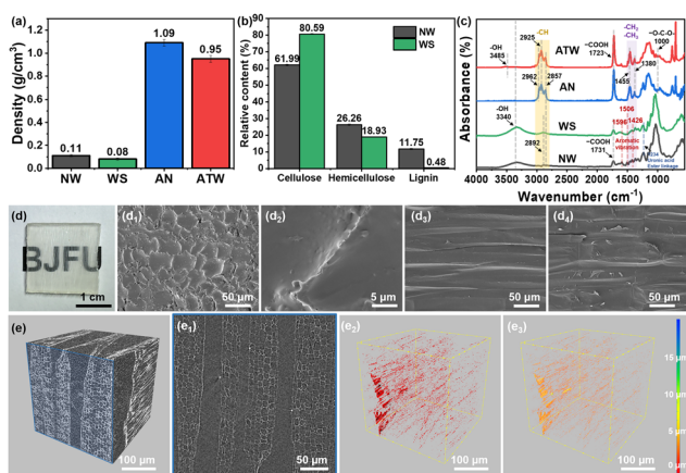
Fig. 2 (a) Density of NW, WS, AN and ATW. (b) Composition contents of cellulose, hemicellulose and lignin for NW and WS. (c) FTIR spectra of NW, WS, AN and ATW. (d) Photograph of ATW: (d 1 )–(d 4 ) transverse (two magnifications), radial, and tangential SEM images of ATW. (e) The μ-CT tomoscan images: (e 1 ) the cross section of ATW; (e 2 ) and (e 3 ) the interfacial porosity distribution in ATW.
