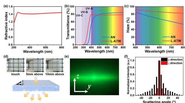
Fig. 3 (a) Refractive index of AN. (b) and (c) Total transmittance and haze of ATW and AN (thickness = 2 mm). (d) Digital images of ATW above the checkerboard pattern. (e) Photograph of the distribution of scattered light spots for ATW. (f) Normalized scattered light intensity distribution for ATW.
