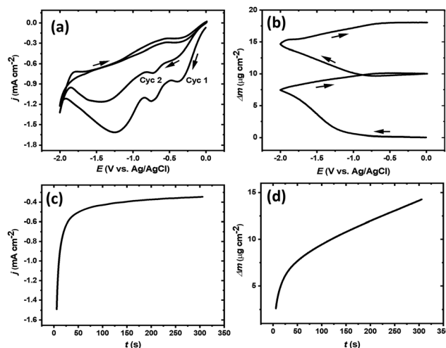
Fig. 2 (a) Two cycles of the CV from 5 mM \text{WSeCl}_4 in MeCN on a Pt-coated quartz electrode. (b) The corresponding mass changes during the CV cycles. (c) Current transients during a potentiostatic deposition at -1.4 V for 5 min on a Pt-coated quartz electrode in EQCM and (d) the corresponding mass change during the potentiostatic deposition. The supporting electrolyte is 0.1 M [\text{Et}_4\text{N}]\text{Cl} and the scan rate is 50 \text{ mV s}^{-1} . Arrows indicate the direction of potential scanning; the starting potential is 0 V.
