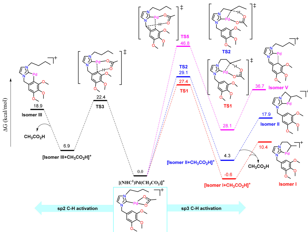
Fig. 7 Computed free energy profile ( \text{kcal mol}^{-1} ) for C–H activation from [(\text{NHC}^1)\text{Pd}(\text{CH}_3\text{CO}_2)]^+ assuming a temperature of 298 K.
