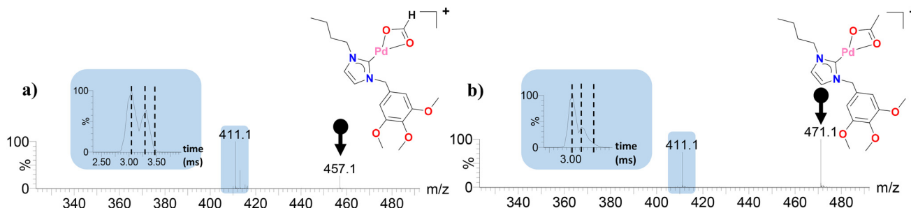
Fig. 2 CID-IM mass spectra of the precursor ions (a) [(\text{NHC}^1)\text{Pd}(\text{HCO}_2)]^+ ( m/z 457.1) and (b) [(\text{NHC}^1)\text{Pd}(\text{CH}_3\text{CO}_2)]^+ ( m/z 471.0) registered at a collision energy of 10 V. The insets show the ATDs of the product ions of formula [(\text{NHC}^1 - \text{H})\text{Pd}]^+ ( m/z 411.1) highlighting the occurrence of three mobility peaks. Note that decarboxylation ( \Delta m = 44 ) 53,54 is also observed as a minor fragmentation channel for the precursor [(\text{NHC}^1)\text{Pd}(\text{HCO}_2)]^+ .
