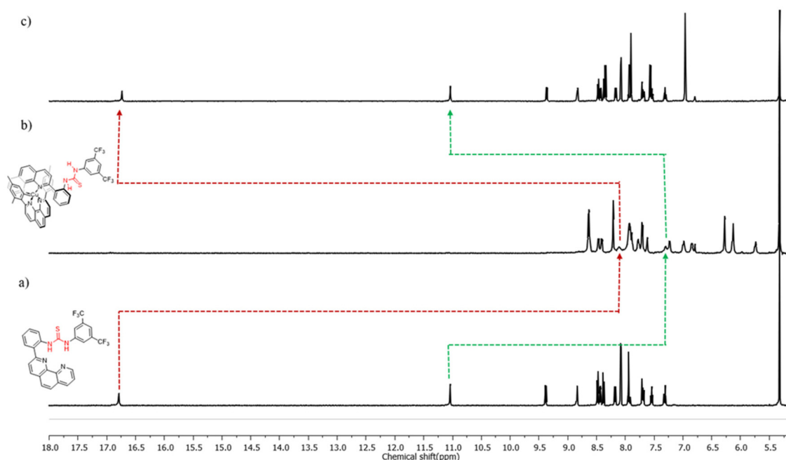
Fig. 4 ^1\text{H} NMR (CD _2 Cl _2 , 298 K, 500 MHz) spectra of (a) switch 1 (10 mM); (b) [\text{Cu}(\textbf{1})(\textbf{3})]\text{PF}_6 ; and (c) [\text{Cu}(\textbf{1})(\textbf{3})]\text{PF}_6 + excess aqueous KCN.
