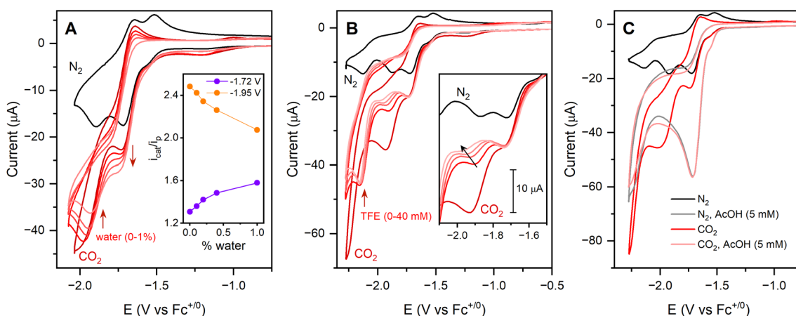
Fig. 8 Catalytic CVs of Re2 (1 mM) in CO 2 -saturated acetonitrile containing three different proton sources: (A) CVs in the presence of increasing amount of water (0%, 0.1%, 0.2%, 0.4%, and 1% v/v). The red trace presents 0% water and current traces with increasing water content is shown by the faded red traces. The inset figure shows the i_{\text{cat}}/i_{\text{p}} ratio variation with water content at the two reduction steps. (B) CVs in the presence of trifluoroethanol (0, 10, 20, 30, and 40 mM with the red trace presenting 0% water) The inset figure shows the shift of the peak potential of the second reduction step with incremental addition of TFE. (C) CVs under N 2 and CO 2 in the presence and absence of acetic acid (5 mM). All voltammograms were recorded at a 100\text{ mV s}^{-1} scan rate in 0.1\text{ M } n\text{-Bu}_4\text{BF}_4 supporting electrolyte.
