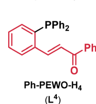
Fig. 1 Hybrid phosphine-EWO ligands used in this work with the chalcone group highlighted in red. A) Fluorinated derivatives (*L 3 has not been previously reported). B) Non-fluorinated Ph analogue.
