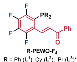
Fig. 1 Hybrid phosphine-EWO ligands used in this work with the chalcone group highlighted in red. A) Fluorinated derivatives (*L 3 has not been previously reported). B) Non-fluorinated Ph analogue.
