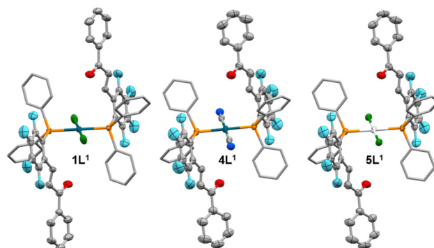
Fig. 2 X-ray structures of 1\text{L}^1 , 4\text{L}^1 and 5\text{L}^1 . H atoms omitted for clarity. Relevant distances in Å: 1\text{L}^1 : Pd–Cl = 2.2903(7), Pd–P = 2.3231(7), C=C (olefin) = 1.314(4). 4\text{L}^1 : Pd–C = 1.990(4), Pd–P = 2.3388(10), C=C (olefin) = 1.320(6). 5\text{L}^1 : Pt–Cl = 2.3029(11), Pt–P = 2.3241(11), C=C (olefin) = 1.303(7).
