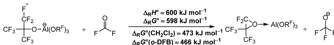
Scheme 1 Calculated isodesmic reaction enthalpies \Delta_{\text{R}}H^\circ and Gibbs free energies \Delta_{\text{R}}G^\circ for the decomposition of the [\text{Al}(\text{OR}^{\text{F}})_4]^- WCAs ((1) and (2) \text{R}^{\text{F}} = \text{C}_{10}\text{F}_{15} ), (3) ( \text{R}^{\text{F}} = \text{C}(\text{CF}_3)_3 ) under fluoride ion abstraction (BP86/def-SV(P) level with D3(BJ) dispersion). Solvation effects on the Gibbs free energy \Delta_{\text{R}}G^\circ were considered by using the COSMO solvation model for \text{CH}_2\text{Cl}_2 ( \epsilon = 8.93^{52} ) and o -DFB ( \epsilon = 13.38^{52} ). The red star marks the abstracted fluoride ion. The experimental FIA of \text{COF}_2 of 209 \text{ kJ mol}^{-1} was used as an anchor point for comparison.
