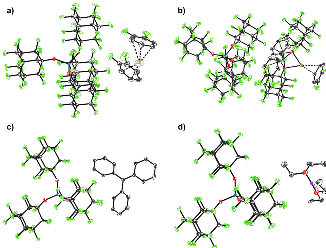
Fig. 2 Molecular structures of the structurally characterized [\text{pfAd}]^- salts: (a) [\text{Ag}(\text{o-DFB})_2][\text{Al}(\text{OC}_{10}\text{F}_{15})_4] (2- o -DFB), (b) [\text{Ag}_3(\text{OC}_{10}\text{F}_{15})_2(\text{o-DFB})_3][\text{Al}(\text{OC}_{10}\text{F}_{15})_4] (3), (c) [\text{Ph}_3\text{C}][\text{Al}(\text{OC}_{10}\text{F}_{15})_4] (4), (d) [\text{H}(\text{OEt}_2)_2][\text{Al}(\text{OC}_{10}\text{F}_{15})_4] (7). Hydrogen atoms are omitted for clarity with the exception for the acidic, bridging proton in (d) (purple). Disorders are omitted for clarity for (a) and (b) as well as two further o -DFB molecules with an occupation number of 4% in (b). The main occupation numbers are presented here. Thermal displacement ellipsoids were drawn at the 50% probability level. For details see ESI.†
