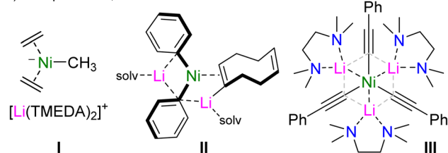
b) Examples of \text{Ni}_2 -ates with benzyne or alkyne ligands
