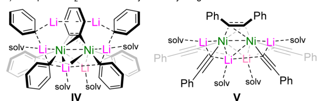
c) This work: \text{Ni}_2 - and \text{Ni} -ates with diphenylacetylene ligands
