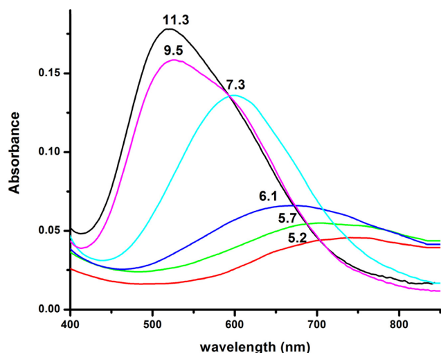
Fig. 8 Visible absorption spectra of the solutions of Cu(II) and R1 (Cu(II) : R1 = 1 : 1.2, T = 298 \text{ K} , I = 0.1 ( \text{KNO}_3 )), recorded at the indicated pH values.
