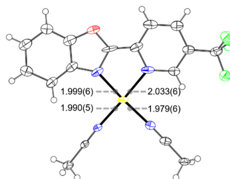
Fig. 4 Single crystal X-ray structure of [Pd(5-CF 3 -PBO) 2 ](MeCN) 2 [Tf 2 N] 2 (CCDC deposition #2094910). The [Tf 2 N] − counter-ions are omitted for clarity. Distances are indicated in Å. Displacement ellipsoids are drawn at the 50% probability level.
