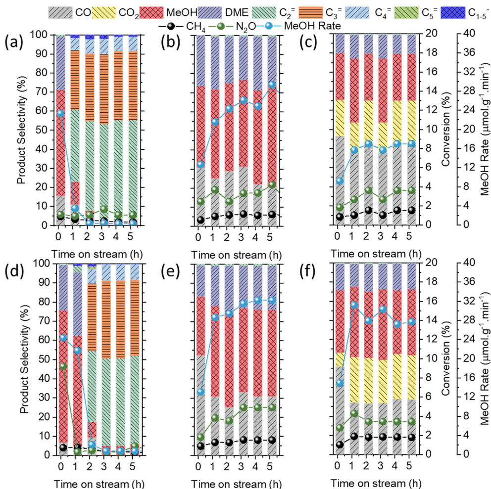
Fig. 5 Stability test of (a) 1Cu/AlEI-C, (b) 5Cu/AlEI-C, (c) 50Cu/AlEI-C, (d) 1Cu/AlEI-S, (e) 5Cu/AlEI-S, and (f) 50Cu/AlEI-S zeolite catalysts in the cDMTM reaction at 350 °C. Reaction conditions: 100 mg catalyst, CH 4 /N 2 O/H 2 O/Ar = 10/10/2/3 ml min -1 , SV = 15 000 ml g -1 h -1 .
