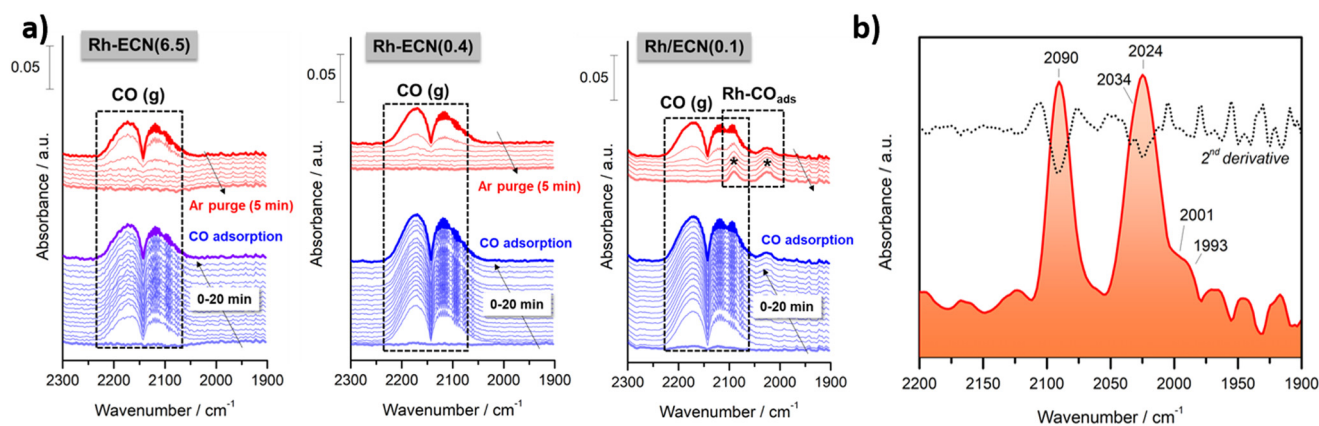
Fig. 3 a) Evolution of in situ DRIFTS spectra during CO adsorption (20 min) and subsequent Ar purging (5 min) at 50 °C on Rh-ECN(6.5), Rh-ECN(0.4) and Rh/ECN(0.1) samples. b) DRIFTS spectra recorded on Rh/ECN(0.1) sample after CO adsorption (20 min) and Ar purging (5 min) at 50 °C. The inclusion of second derivative curve facilitates the identification of the bands.
