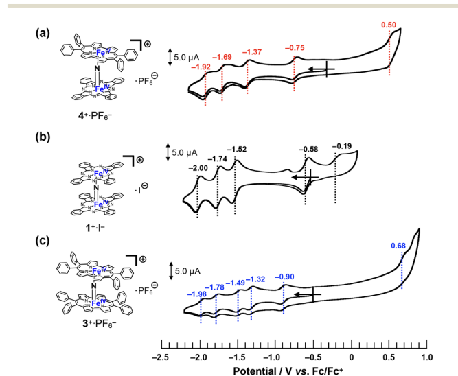
Fig. 5 Comparison of cyclic voltammograms of (a) 4^+\cdot\text{PF}_6^- , (b) 1^+\cdot\text{I}^- , and (c) 3^+\cdot\text{PF}_6^- in a pyridine solution containing 100 mM of ^n\text{Bu}_4\text{N}^+\cdot\text{PF}_6^- at room temperature. [Substrate] = 200 \mu\text{M} , [scan rate] = 100 \text{mV s}^{-1} .
