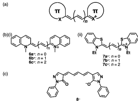
Fig. 4 (a) General structure of polymethine dyes, (b) positively charged polymethine dyes based on (i) N -methylquinolinium ( 6a -c + ) (ii) benzothiazolium ( 7a -c + ) and (c) negatively charged polymethine dye based on deprotonated oxonol ( 8 - ).
