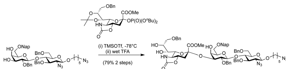
Scheme 14 Regioselective glycosylation with sialic acid dibutyl phosphate. 16
