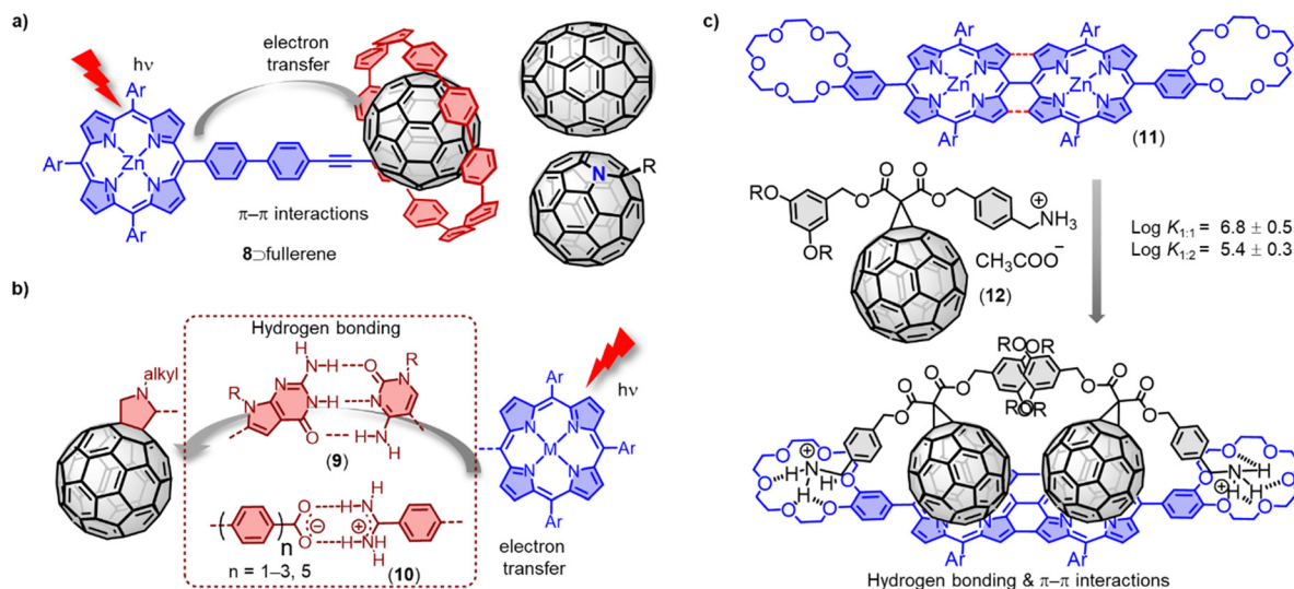
Fig. 7 (a) Efficient electron transfer in modular 80 fullerene complexes. (b) Selected examples of hydrogen bond bridged C 60 -based D-A dyads (9 and 10) and corresponding charge transfer process. (c) Supramolecular complexation between ditopic porphyrin receptor 11 and fullerene derivative 12.
