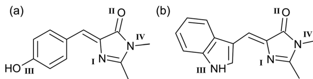
Fig. 1 Structure of (a) pHBDI and (b) Cyan. The protonated cations are denoted pHBDI + and Cyan + , with the four possible protonation sites identified. In both cases, protonation site I (imine) corresponds to the lowest energy protomer. Each protomer may have E and Z geometric configurations about the double bond on the methine bridge. In all cases, the Z isomer is lower in energy. The E isomer, if present, is expected in only trace quantities.
