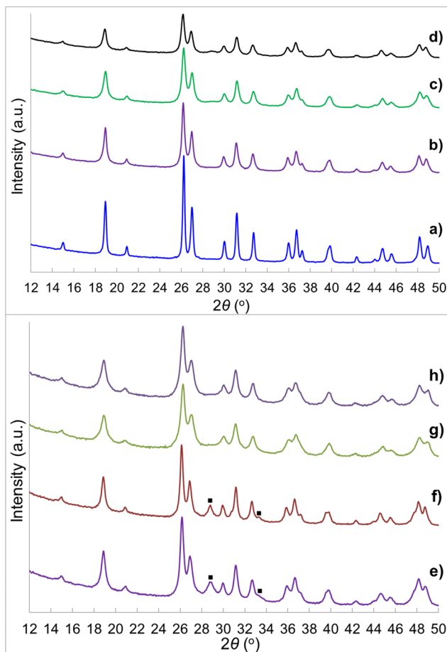
Fig. 2 XRD patterns of samples (a) w0, (b) \phi 12w1-4, (c) \phi 12w1-2, (d) \phi 12w3-4, (e) \phi 8w1-2, (f) \phi 8w3-4, (g) \phi 20w1-2, (h) \phi 20w3-4, (■) CeO 2 . Sample details are shown in Tables 2 and 3.
