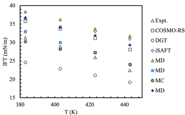
Fig. 9 Benchmark and predicted interfacial tensions for the water/50 : 50 n -dodecane + toluene mixture. The uncertainty is of the order of 1 \text{ mN m}^{-1} for the experimental data and approx. 0.5\text{--}3 \text{ mN m}^{-1} for the predictive methods. Adapted with permission from ref. 77. See original source for the full discussion of the methods and force-fields used. Copyright 2018 Elsevier.
