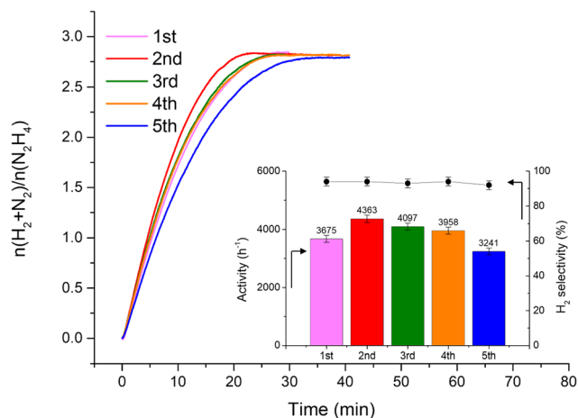
Fig. 3 Stability tests for 1 wt% Ir/GCN. The insets are the catalytic activity (left axis) and \text{H}_2 selectivity (right axis) trends along repeated cycles. All tests were performed at 323 K and 1400 rpm, using 300 \mu\text{L} of a 3.3 M hydrazine solution in 5 mL of 0.5 M NaOH and a \text{N}_2\text{H}_4 \cdot \text{H}_2\text{O} :catalyst molar ratio of 1000:1. A sampling time of 0.3 s was employed to obtain continuous kinetic profiles.
