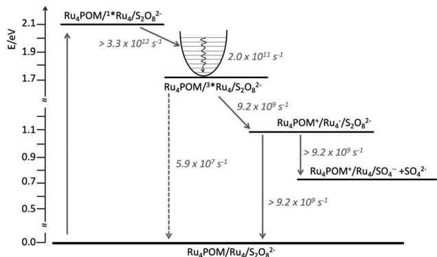
Fig. 8 Energy level diagram and schematization of the processes (and rate constants) occurring upon excitation of Ru4 in the Ru4POM/Ru4/ \text{S}_2\text{O}_8^{2-} system (solid and dashed lines refer to nonradiative and radiative processes, respectively). For further details, see ref. 17.
