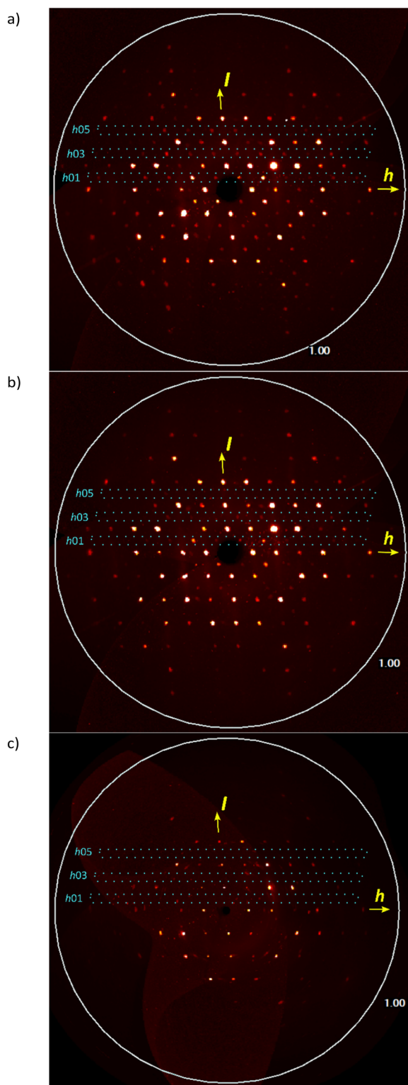
Fig. 8 Pseudo ( h0l ) precession images for (a) the room temperature reacted crystal at \sim 64\% (just before transformation), and after the P\bar{1} to C2/c transformation at (b) \sim 79\% and (c) \sim 89\% conversion. The ( h01 ), ( h03 ), and ( h05 ) reflections enclosed with dotted lines are allowed in the triclinic P\bar{1} space group (a) but are weaker in (b) and absent in (c) as required for C2/c .
