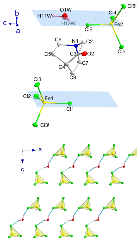
Fig. 4 (Top) View of a fragment of B obtained from the refinement at 100 K, including the atoms from the asymmetric unit and those generated by the application of the mirror planes (highlighted in blue; I: x, 1/2 - y, z , II: x, 3/2 - y, z ) to complete the iron environment (non-H atoms with ellipsoids at 50% of probability). The hydrogen atoms of the organic unit have been omitted for the sake of clarity. (Bottom) Detail of the inorganic layers extended on the ac -plane for B . The \text{Cl}\cdots\text{H}-\text{O} hydrogen bonds have been highlighted through dashed blue lines.
