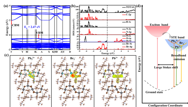
Fig. 4 (a) Calculated electronic band structures and (b) DOS of (HM)Pb 2 Br 6 . (c) Calculated charge density for (HM)Pb 2 Br 6 (Pb 2 3+ , Br 2 − and Pb 3+ STLs holes) upon crystal lattice perturbation via the Pb–Pb, Br–Br and Pb–Br distances shortening. (d) Configuration coordinate diagram illustrating the luminescence mechanism.
