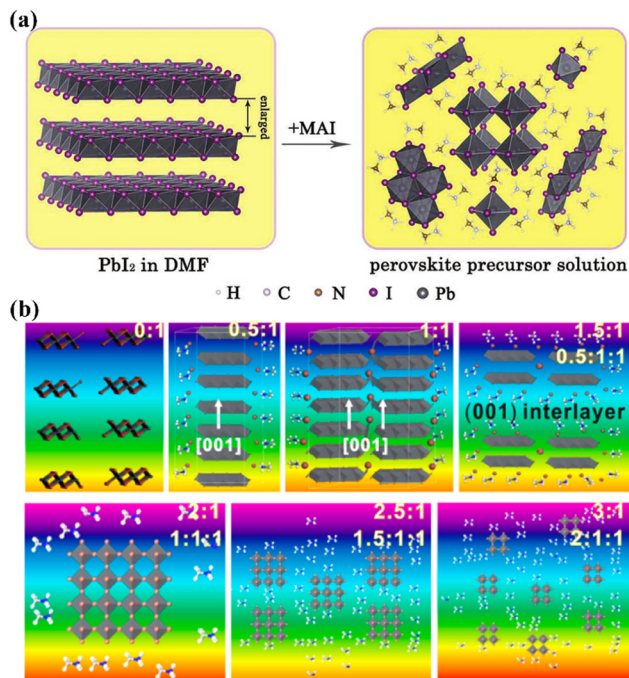
Fig. 3 (a) Schematic of the evolution of lead-iodine complexes after MAI addition. 53 Copyright 2019, Wiley-VCH Verlag. (b) Types of lead iodine complexes that may occur in precursors with different MAI/ PbI_2 mole ratios. 55 Copyright 2015, American Chemical Society.
