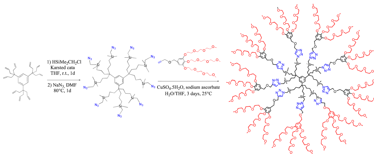
Scheme 16 Synthesis of a dendritic unimolecular micelle as template for multiple catalytic uses (molecular catalysis with Grubbs II catalyst, metal ion click catalysis with \text{Cu}(\text{I}) , and nanoparticle catalysis).
